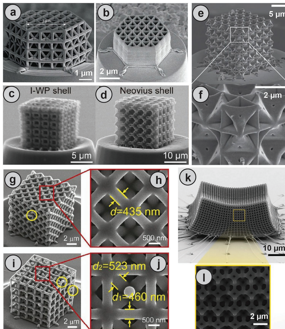
Figure 5. Examples of DLW-fabricated nanoarchitected 3D PyC metamaterials based on different unit cells: a) tetrahedron, b) triangular, c) Schoen's I-graph-wrapped package (I-WP) shell, d) Neovius shell, e, f) cubic+octet plate, g, h) octet truss, i, j) iso-truss, and k, l) tetrakaidecahedron. (a, b) are reprinted with permission. [85] Copyright 2016, Springer Nature. c and d are reprinted with permission. [88] Copyright 2022, National Academy of Sciences. (e, f) are reprinted with permission. [87] Copyright 2020, Springer Nature. (g–j) are reprinted with permission. [86] Copyright 2019, National Academy of Sciences. (k, l) are reprinted with permission. [90] Copyright 2021, Springer Nature.
