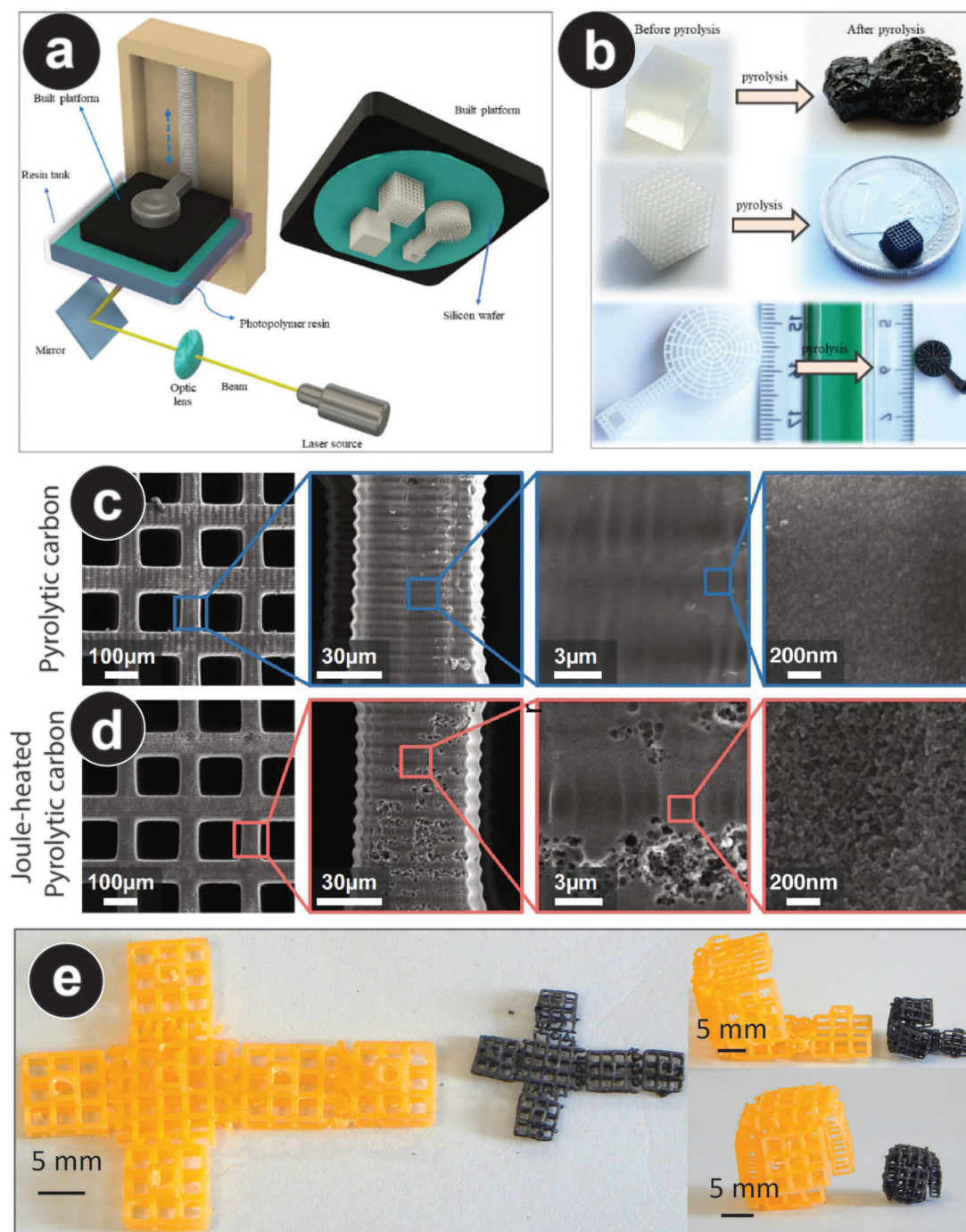
Figure 4. a) Schematic illustration of a typical SLA-based 3D printing system. b) SLA-printed bulk (top row) and architected structures (middle and bottom row) before and after pyrolysis, showing architected structure retaining the precursor geometry, unlike the bulk material. (a,b) are reprinted with permission. [30] Copyright 2020, Elsevier. Surface porosity of SLA-printed c) PyC and d) joule-heated PyC, showing the higher surface porosity of the joule-heated PyC material. Reprinted with permission. [42] Copyright 2020, Springer Nature. e) Sequential configurations of a shape-morphing SLA-printed mechanism before and after carbonization, showing the retention of shape-morphing capabilities of PyC as a feasible approach for fabricating 4D architected PyC. Reprinted with permission. [58] Copyright 2022, Wiley-VCH GmbH.
