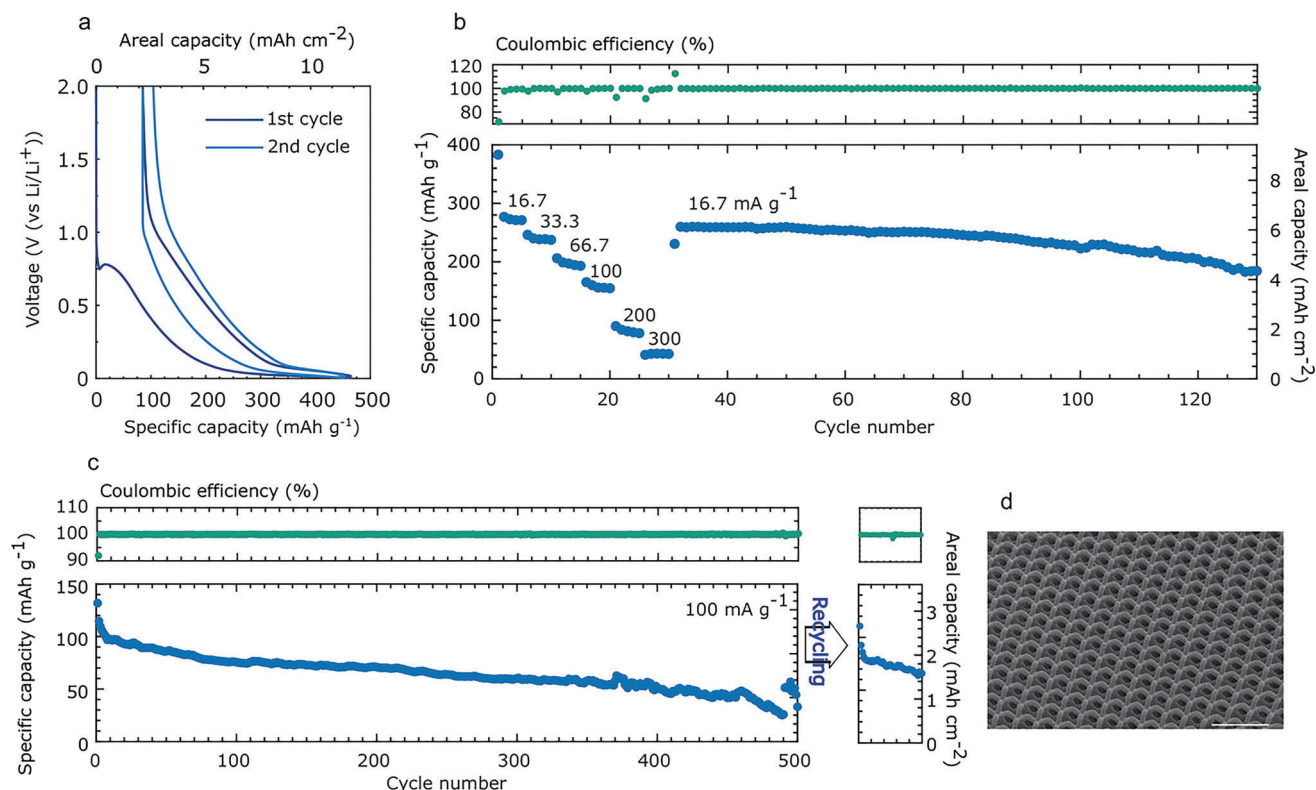
Figure 9. Galvanostatic cycling of microarchitected 3D PyC in a Li-ion battery. a) First two discharge-charge curves at a low current of 2 mA g -1 . b) Coulombic efficiency (top) and discharge capacities (bottom) at step currents. c) Specific capacitance and coulombic efficiency for 500 cycles at 100 mA g -1 . d) SEM image of a representative microarchitected 3D PyC electrode after >300 cycles at 100 mA g -1 . Scale bar is 500 μm for (d). Reprinted with permission. [96] Copyright, 2021 Wiley-VCH GmbH.
