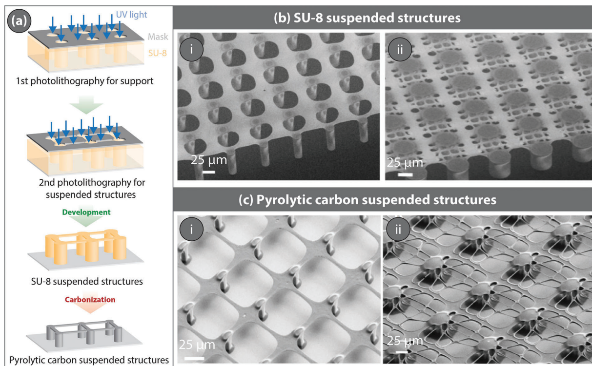
Figure 3. a) Schematic illustration of the multistep photolithography process leading to the fabrication of suspended pyrolytic carbon structures. b) Examples of suspended SU-8 structures, and c) their corresponding carbonized structures. Carbonization of (b,i,ii) leads to (c,i,ii), respectively. It should be noted how the carbonization-assisted shrinkage led to the stretching of the suspended structures after carbonization. (b,c) are reprinted with permission. [49] Copyright 2016, Institute of Physics.
