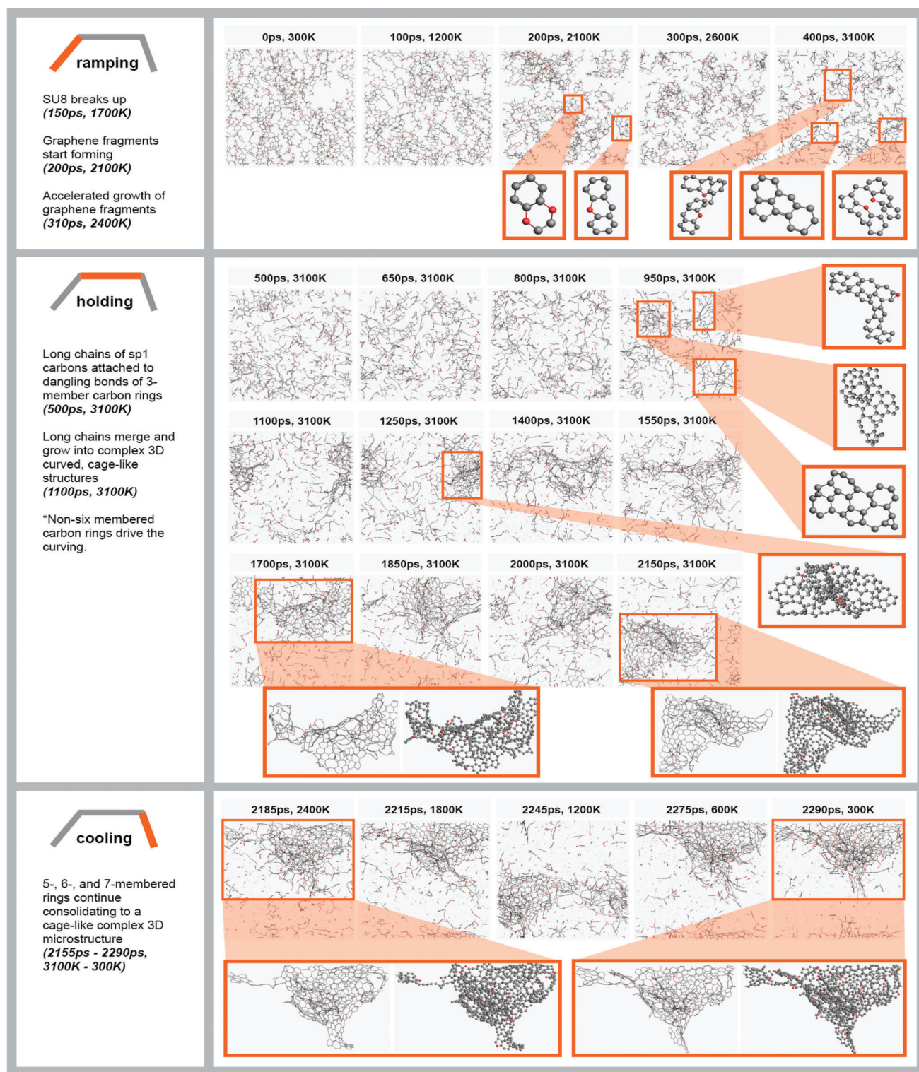
Figure 2. Results from Reactive Molecular Dynamic Simulations of the pyrolysis of SU-8 epoxy resins, showing the molecular transformation at the different stages of pyrolysis. The black spheres represent carbon atoms, whereas the red spheres are oxygen atoms. Note that the temperature employed in this simulation study is much higher than that used in a typical pyrolysis process for PyC (3100 K in simulation vs 900°C in experiments) to accelerate the process in simulations, allowing the reaction energy barriers to overcome easily. Reprinted with permission. [36] Copyright 2021, Elsevier.
