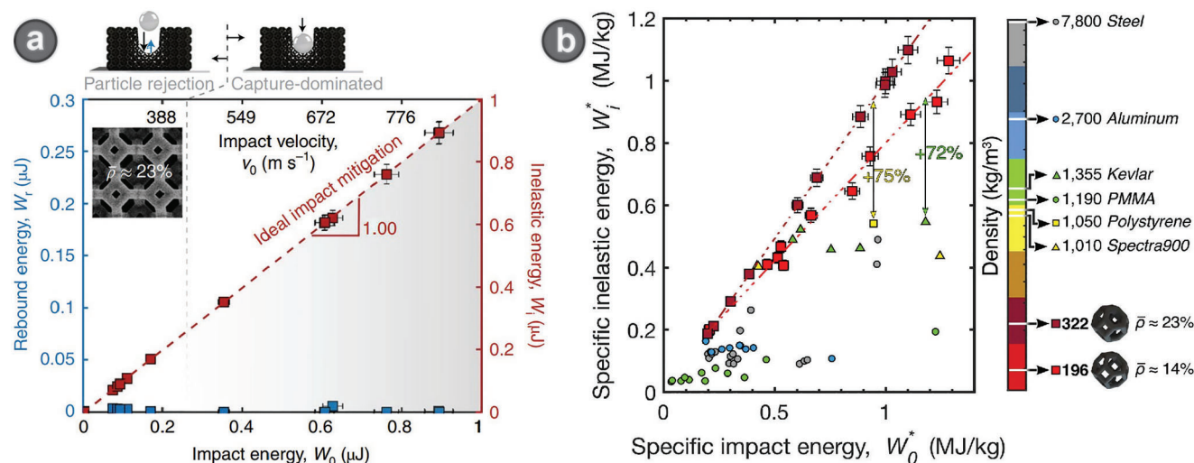
Figure 7. a) Impact energetics for supersonic impact experiments on nanoarchitected 3D PyC metamaterial, featuring a tetrakaidecahedron unit cell shown in Figure 5k,l and \bar{\rho} \approx 23\% , demonstrating two regimes upon the high-speed impact of a \text{SiO}_2 microsphere: formation of crater and rejection of the microsphere, and partial penetration and particle capture. The inelastic energy or the impact resistance energy fits linearly with a slope of 1 with the impact energy, showing excellent energy absorption. b) Comparison of specific inelastic energy (=inelastic energy/mass of the participant material) of nanoarchitected 3D PyC with other traditionally used impact-resistant materials with specific impact energies (=impact energy/mass of the participant material). It shows significant improvement in specific impact resistance in the case of nanoarchitected 3D PyC. Both the figures are reprinted with permission. [90] Copyright 2021, Springer Nature.
